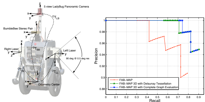
Figure 2. Robotic platform (left) with a cross-calibrated lidar-camera system yielding inter-word 3D distances. Precision-recall curves (right) for the New College data set. FAB-MAP 3D has a higher recall of 74% at 100% precision than FAB-MAP which has 42% recall at 100% precision. The accelerated approach has marginally lower recall of 71% but still performs better than FAB-MAP.
